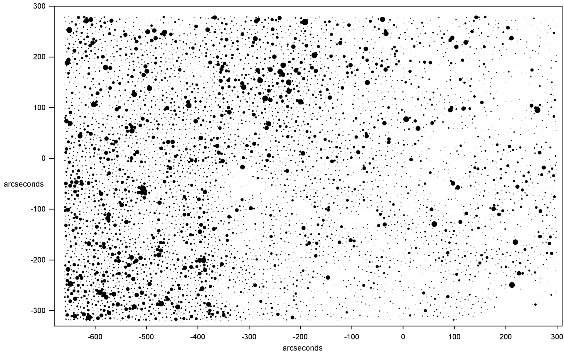
Grid PRF (Dphot) Photometry for WISE , David G. Elliott, JPL, delliott3@charter.net . This plot shows stars measured from WISE W1 (3.4 \mu\text{m} ) images of the Galactic Center. North is up, East is left, and the origin is at Sgr A. Dphot fits arrays of PRFs on 2 arcsec spacings to the 13 overlapping WISE images of this area. Positive fits give the source detections shown here.
